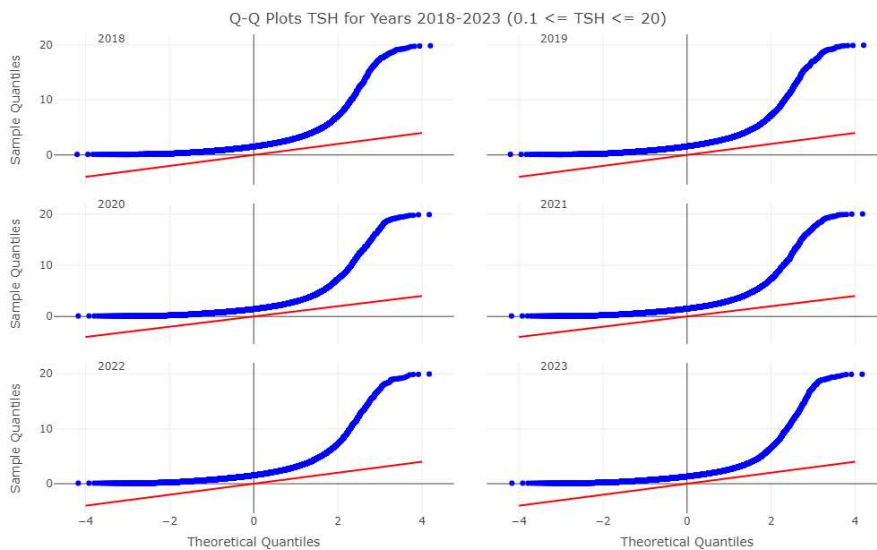
Figure 9. Q-Q plots for all measurements of TSH with values from 0.1-20 \mu\text{U}/\text{mL} of dataset 1 of the corresponding treatment years 2018-2023. N= 208'310 .
