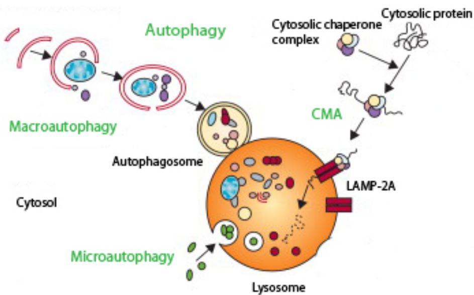
Figure 3. Autophagy system
